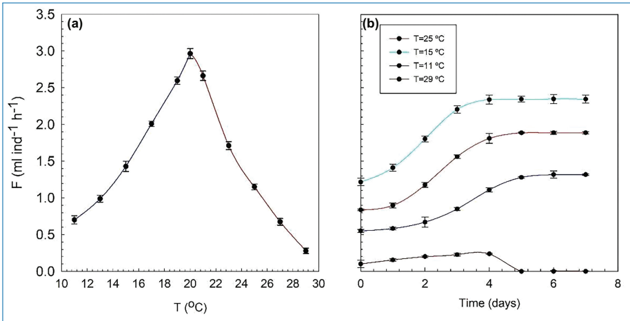
Figure 5.4. (a) D. magna filtration capacity, F ( \text{ml ind}^{-1} \text{h}^{-1} ) versus water temperature and (b) D. magna filtration capacity F ( \text{ml ind}^{-1} \text{h}^{-1} ) during acclimation versus the time (in days) exposed at each water temperature.
