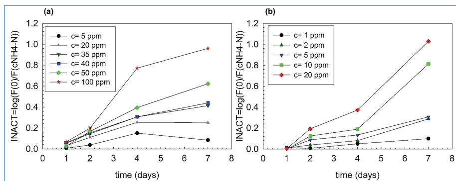
Figure 5.5. Inactivation factor (INACT) versus exposure time (in days) for the different chemical dosages c (in ppm = mg L -1 ) for (a) NH 4 + -N and (b) NO 2 - -N.
