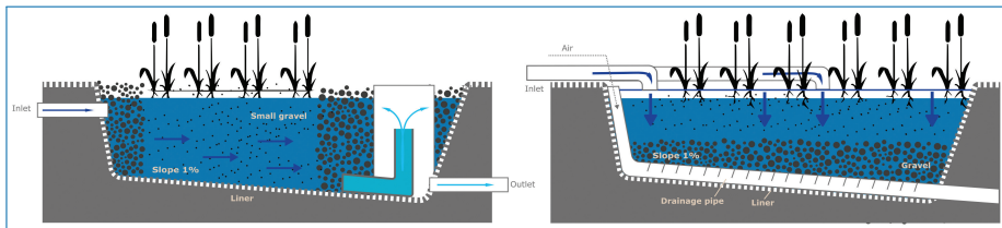
Figure 3.5. Flow path for Horizontal Flow Constructed Wetland (HFCW) and Vertical flow constructed Wetlands (VFCW). Adapted from Gorito et al. (2017) and Tilley et al. (2008).
