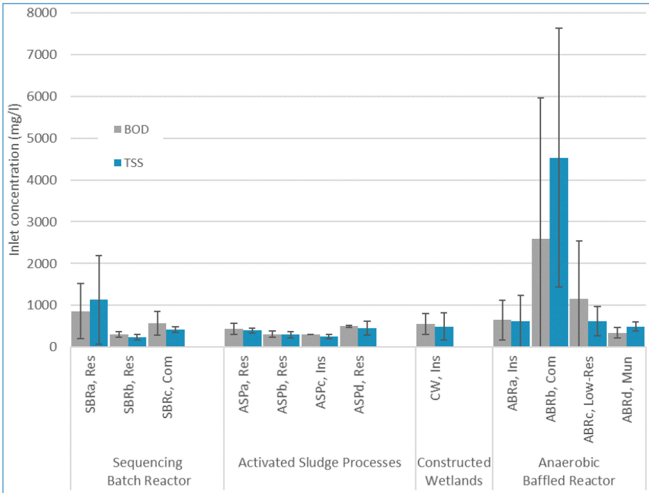
Figure 3.7. Average BOD and TSS influent concentration of small-scale sanitation systems in India. Error bars indicate standard deviations. Approximate values taken from Klinger et al. , 2020.
