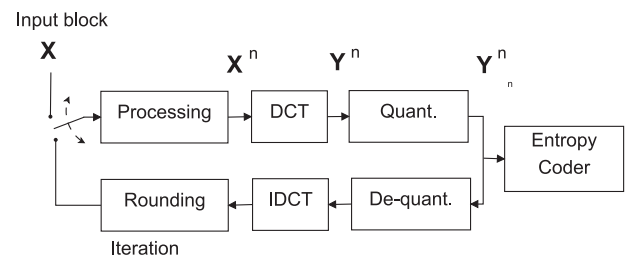
Fig. 1. Block diagram for multiple JPEG compression.
